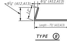
Reinforcement Details
